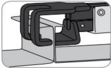
Double angle jaws to clamp 90° flanged, lapped or adjacent joints
