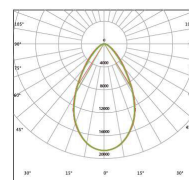
H00212 (60°)
