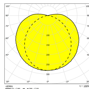
GALGO-LED in symmetrical optics.
