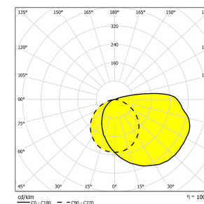
GALGO-LED in asymmetrical optics.
