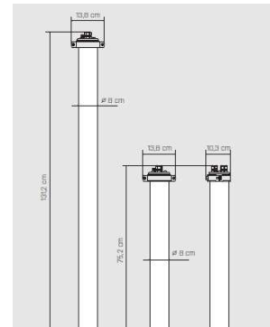
At the end of the luminaire there is a choice in one or two cable glands for easier cable management.
