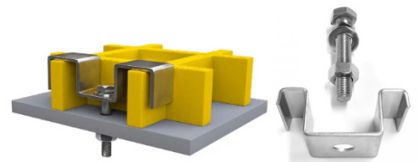
C-Clip
