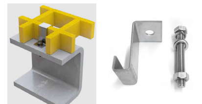
J-Clamp
