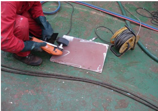
Tercoo® Multi Machine rotating blasting job on a new steel plate.
